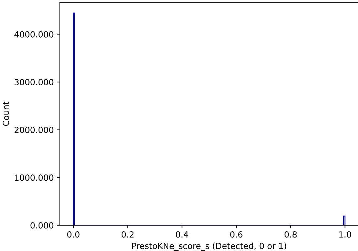
too_combined_s1.0_split_v3.4_10yrs : PrestoKNe_score_s
