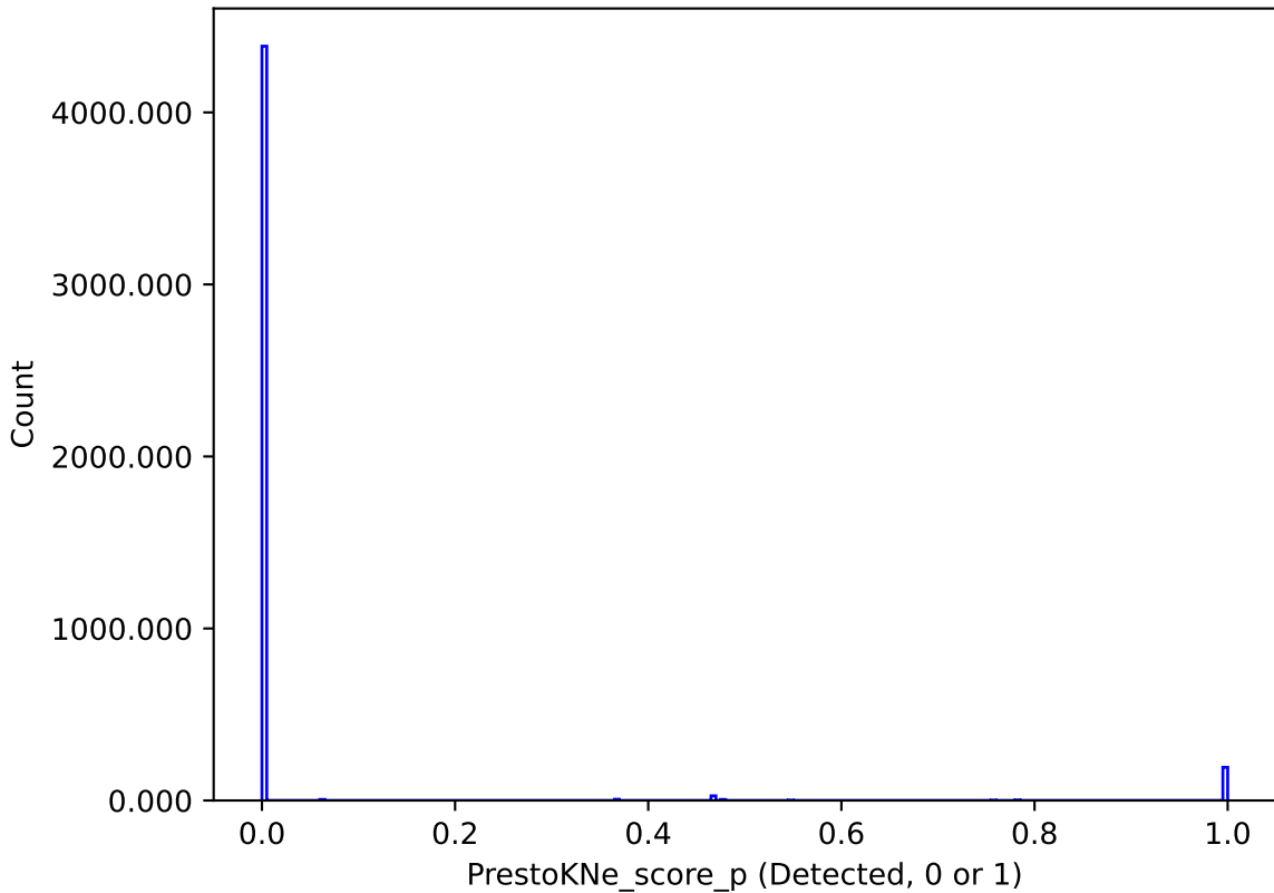
too_combined_s1.0_split_v3.4_10yrs : PrestoKNe_score_p
