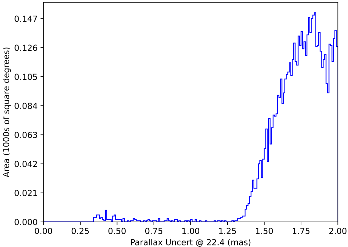
too_combined_s1.0_split_v3.4_10yrs : Parallax Uncert @ 22.4
