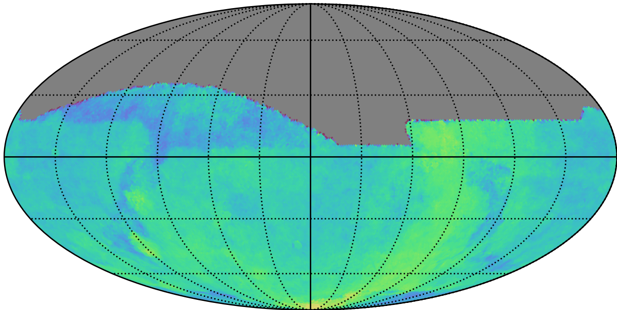
too_combined_s1.0_split_v3.4_10yrs : Parallax Coverage @ 22.4
