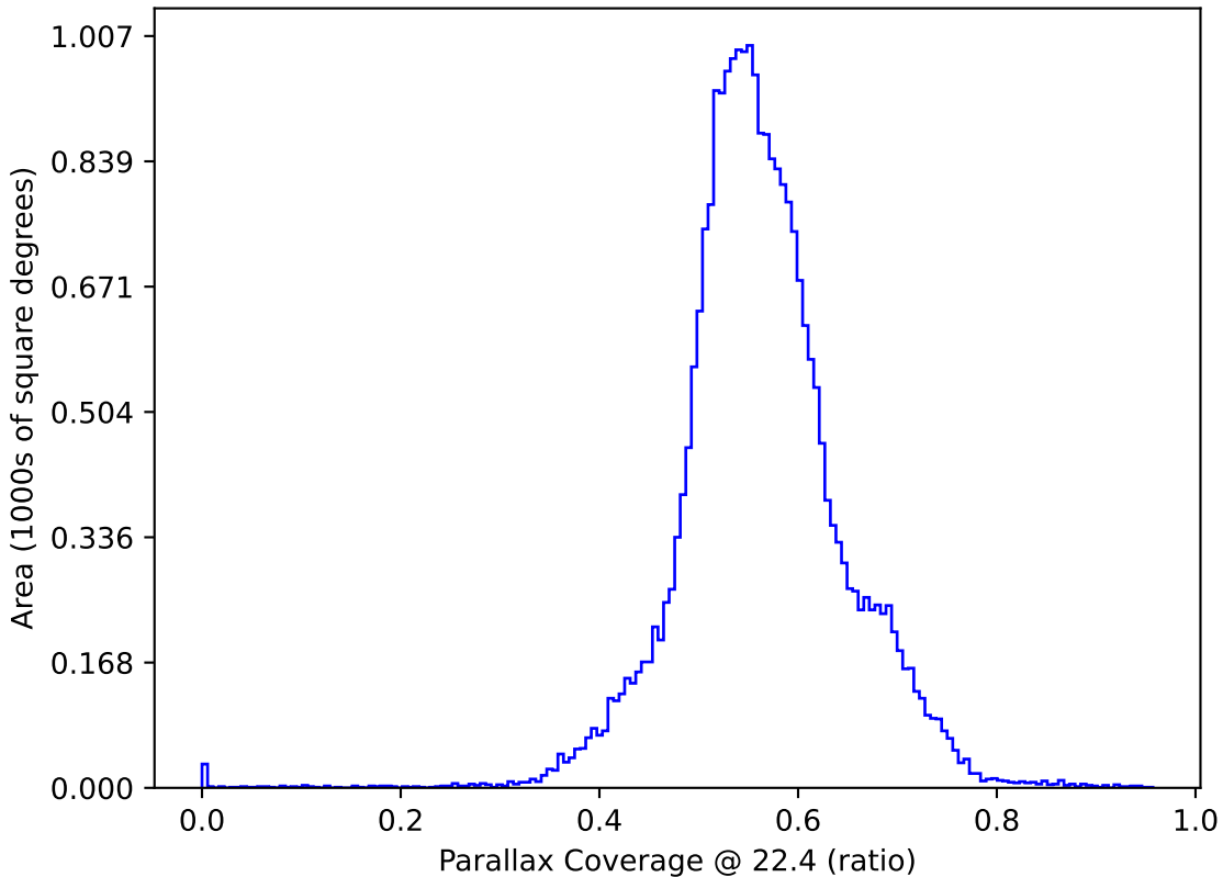
too_combined_s1.0_split_v3.4_10yrs : Parallax Coverage @ 22.4
