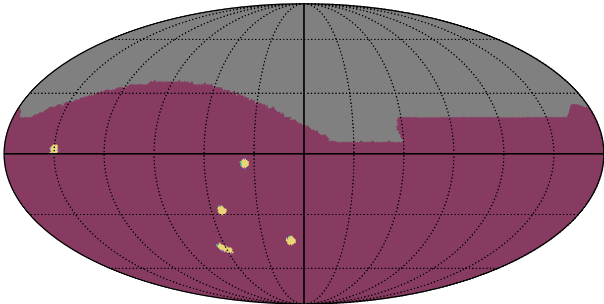
too_combined_s1.0_split_v3.4_10yrs : NumberOfQuickRevisits
