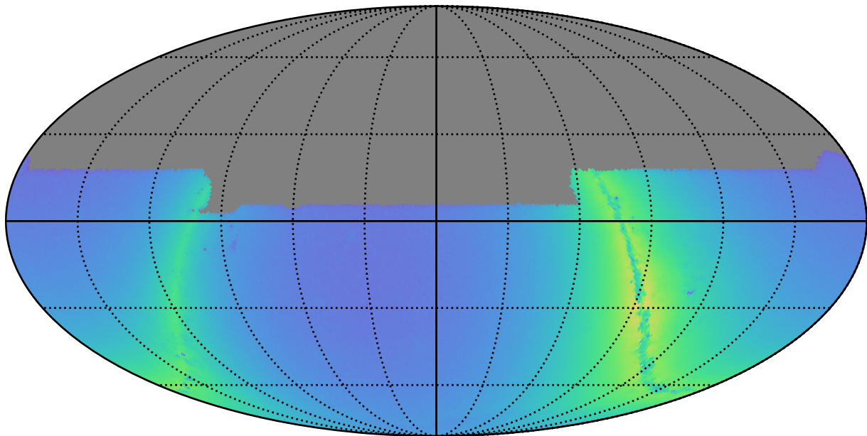
too_combined_s1.0_split_v3.4_10yrs y: Nstars_no_crowding
