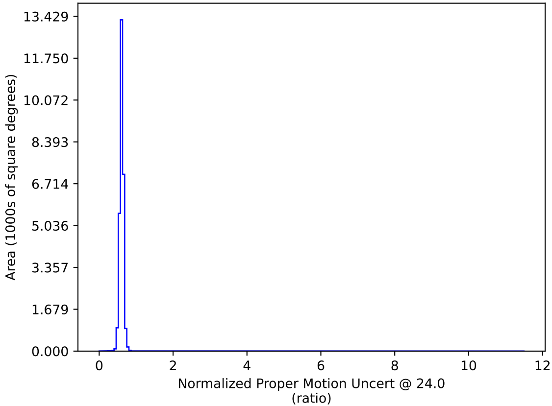
too_combined_s1.0_split_v3.4_10yrs : Normalized Proper Motion Uncert @ 24.0
