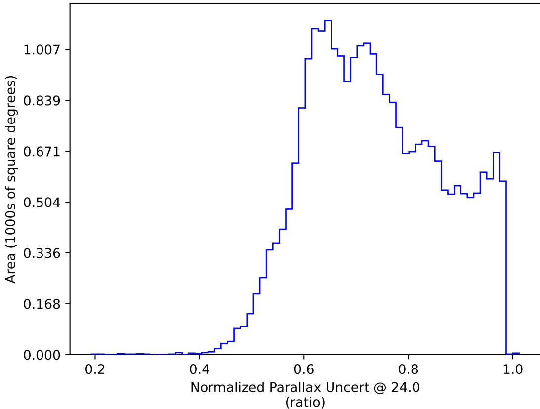
too_combined_s1.0_split_v3.4_10yrs : Normalized Parallax Uncert @ 24.0
