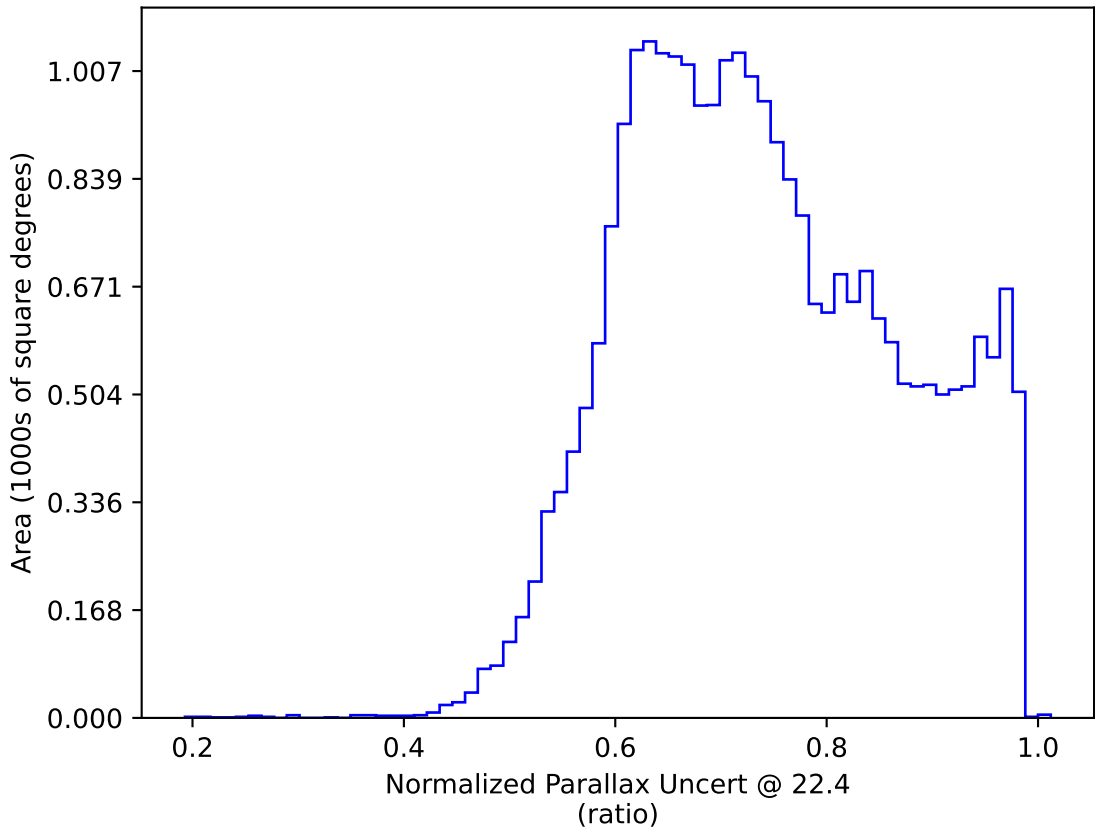
too_combined_s1.0_split_v3.4_10yrs : Normalized Parallax Uncert @ 22.4
