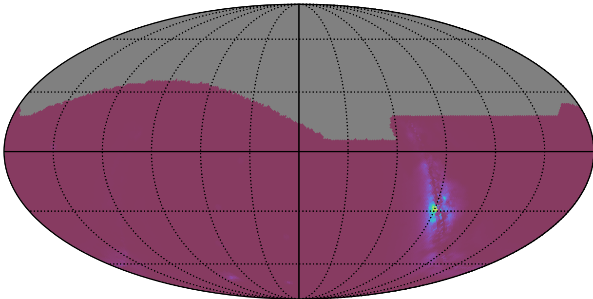
too_combined_s1.0_split_v3.4_10yrs : NlcPoints
