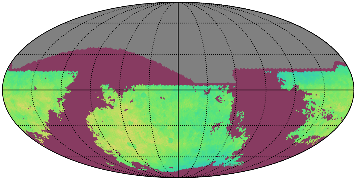
too_combined_s1.0_split_v3.4_10yrs i: NgalScale
