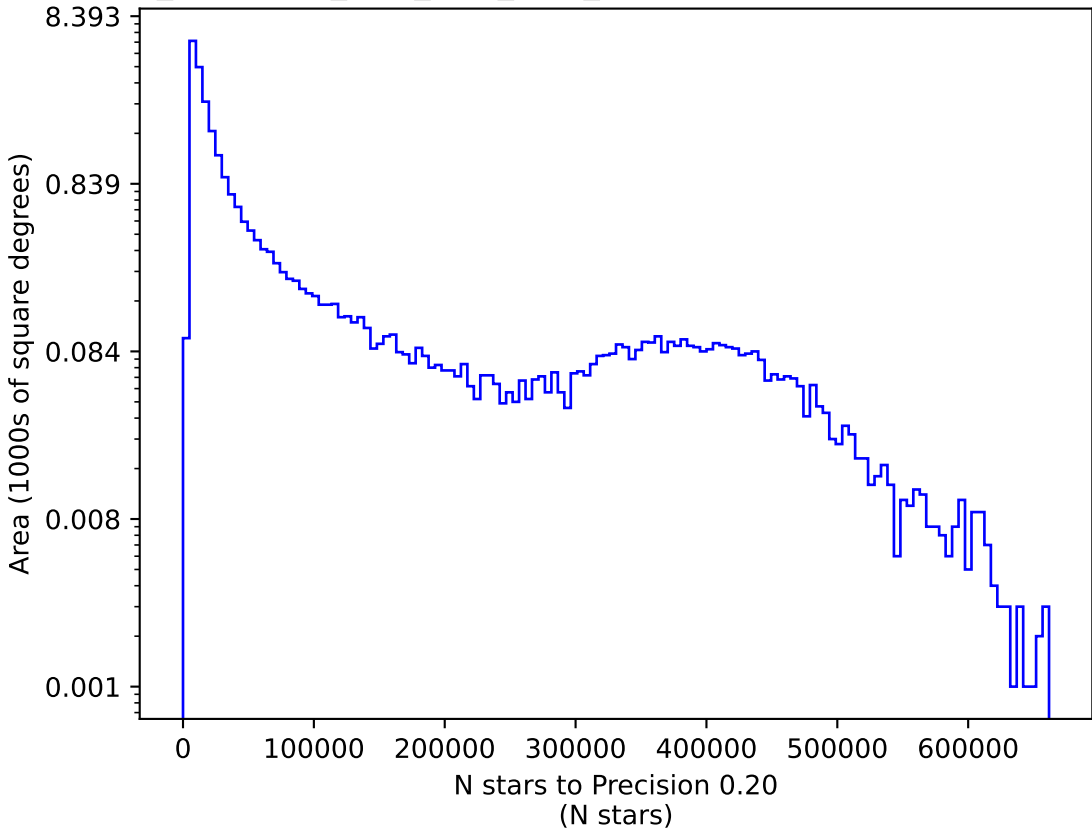
too_combined_s1.0_split_v3.4_10yrs z: N stars to Precision 0.20
