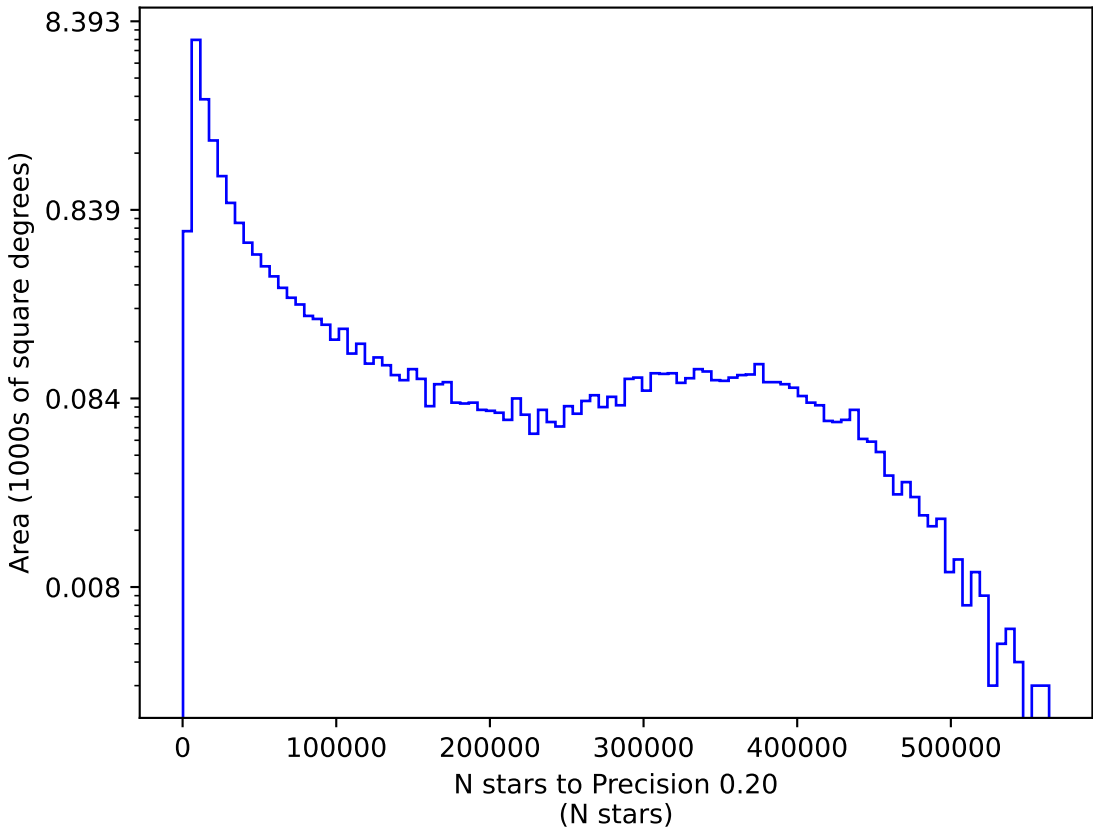
too_combined_s1.0_split_v3.4_10yrs y: N stars to Precision 0.20
