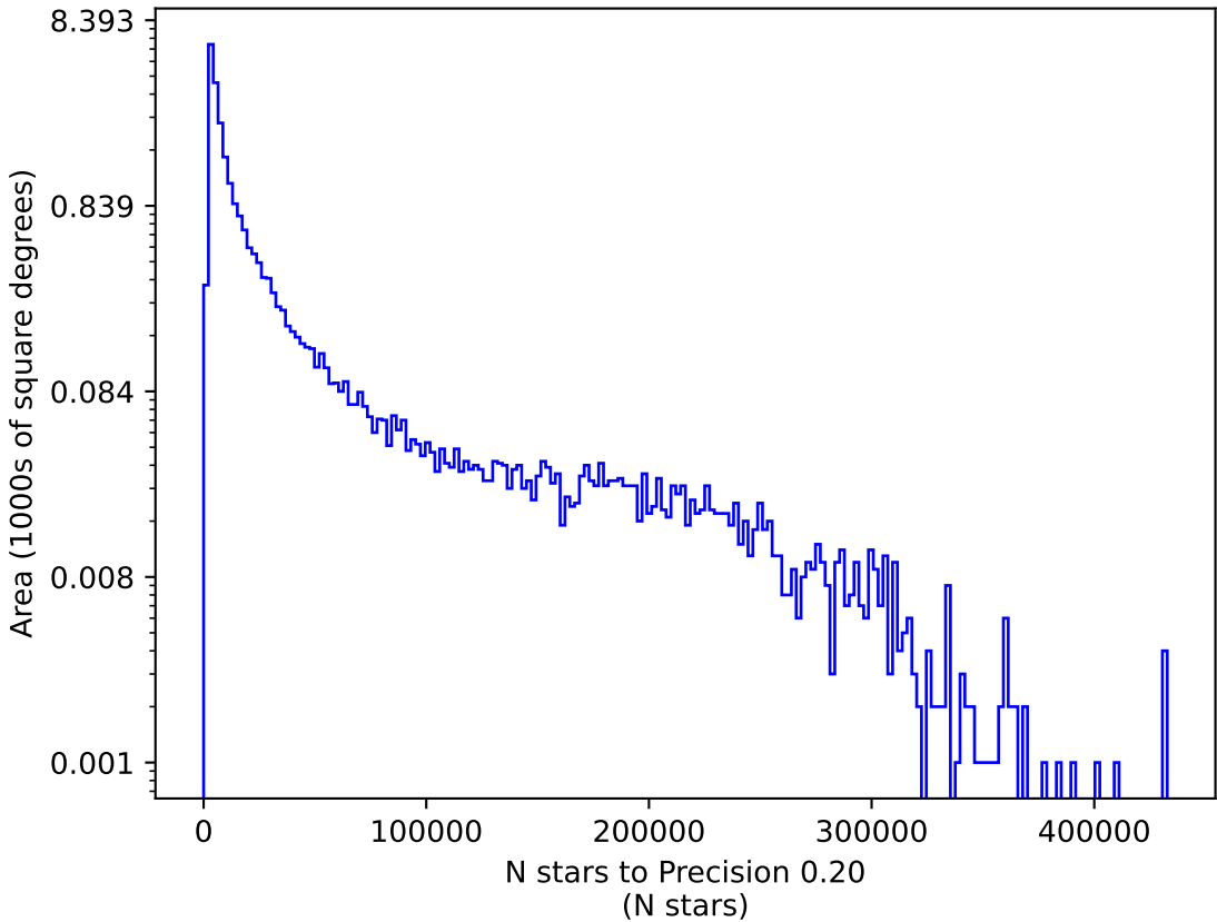
too_combined_s1.0_split_v3.4_10yrs u: N stars to Precision 0.20
