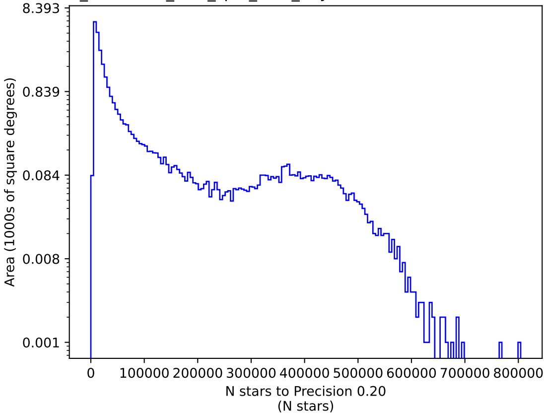
too_combined_s1.0_split_v3.4_10yrs i: N stars to Precision 0.20
