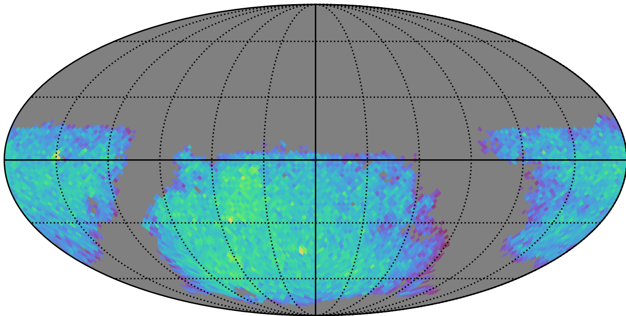
too_combined_s1.0_split_v3.4_10yrs gi: LVDwarfs
