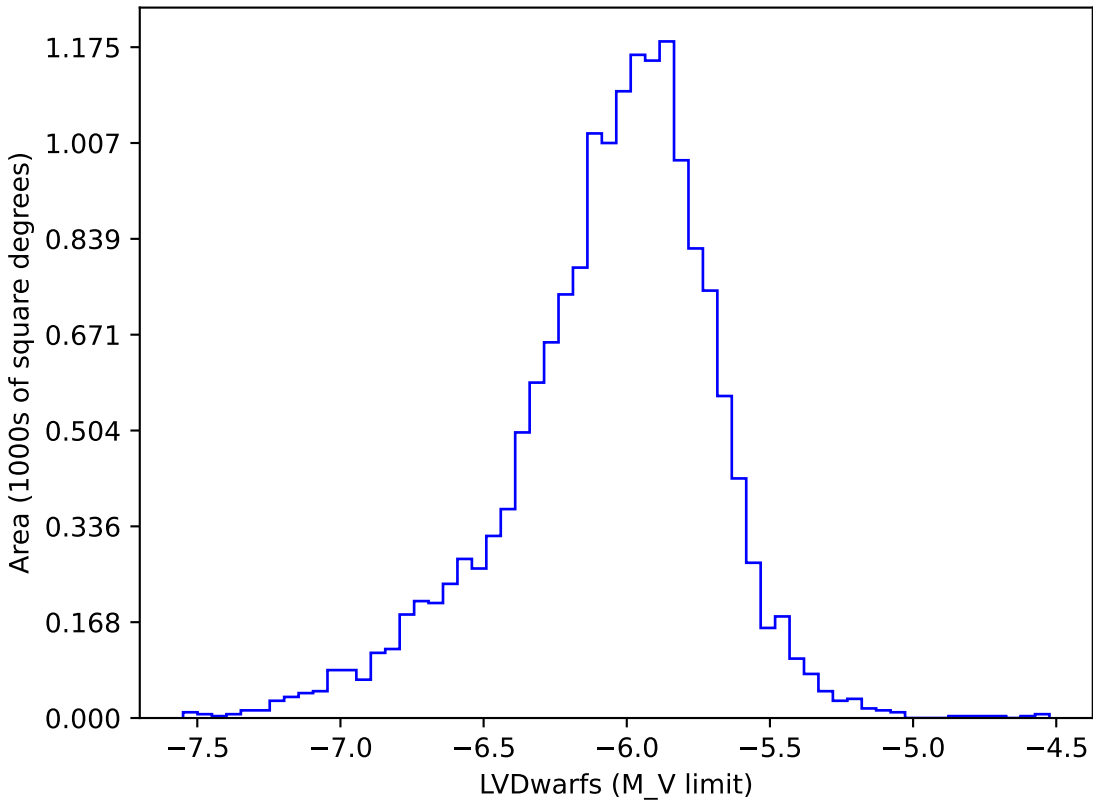
too_combined_s1.0_split_v3.4_10yrs gi: LVDwarfs
