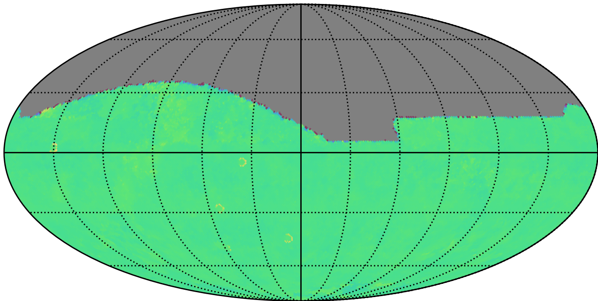
too_combined_s1.0_split_v3.4_10yrs z: Kuiper rotTelPos
