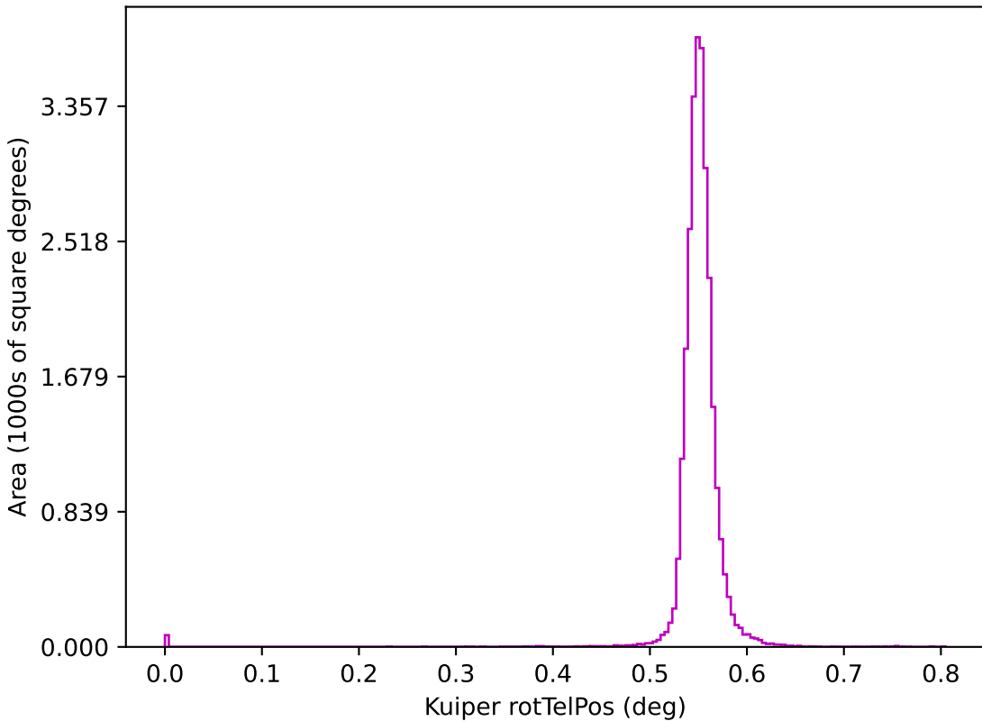
too_combined_s1.0_split_v3.4_10yrs z: Kuiper rotTelPos
