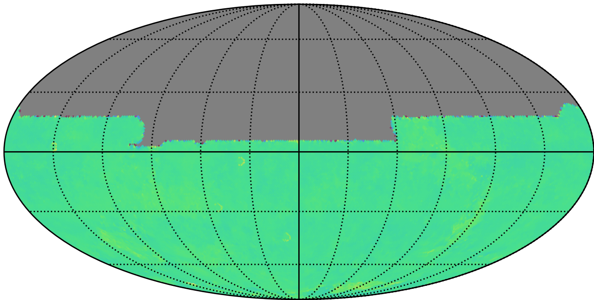
too_combined_s1.0_split_v3.4_10yrs y: Kuiper rotTelPos
