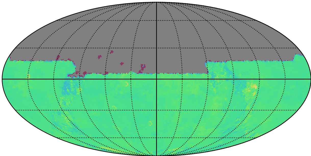
too_combined_s1.0_split_v3.4_10yrs u: Kuiper rotTelPos
