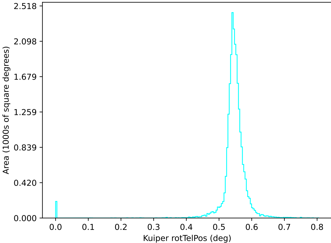
too_combined_s1.0_split_v3.4_10yrs u: Kuiper rotTelPos
