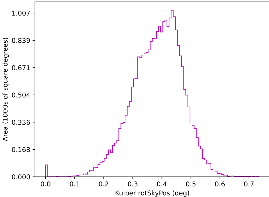
too_combined_s1.0_split_v3.4_10yrs z: Kuiper rotSkyPos
