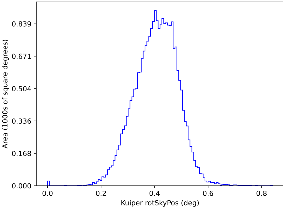
too_combined_s1.0_split_v3.4_10yrs y: Kuiper rotSkyPos
