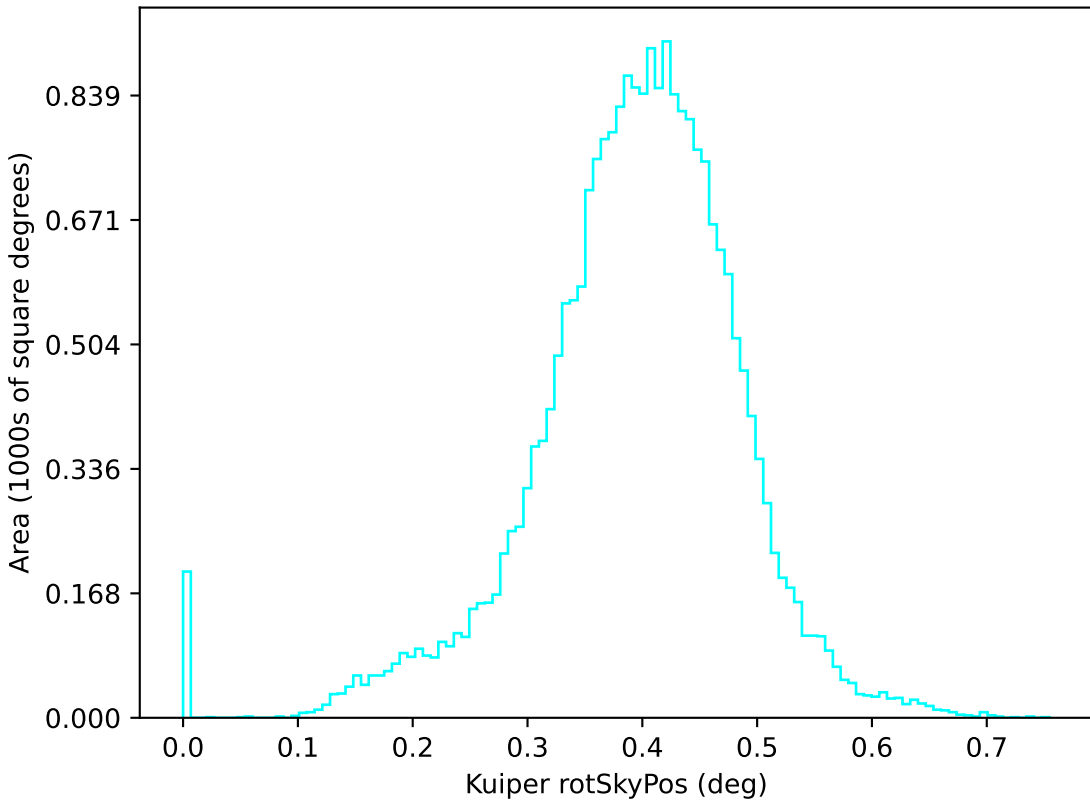
too_combined_s1.0_split_v3.4_10yrs u: Kuiper rotSkyPos
