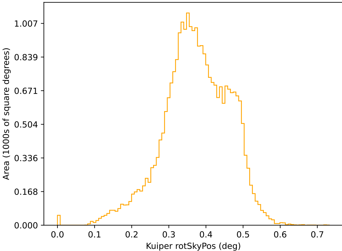
too_combined_s1.0_split_v3.4_10yrs r: Kuiper rotSkyPos
