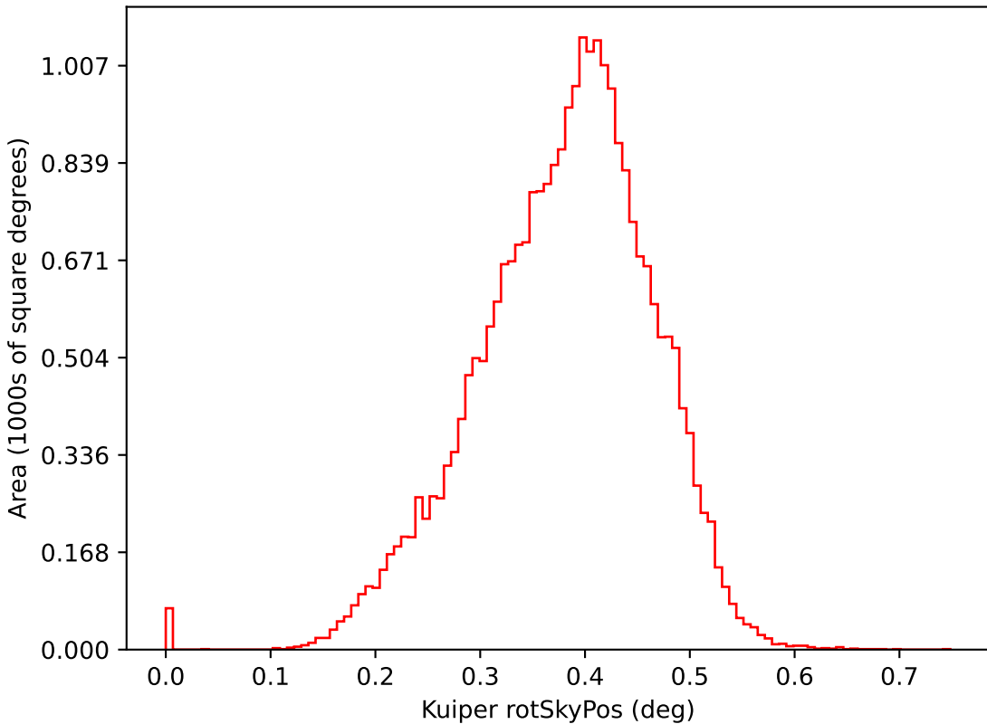
too_combined_s1.0_split_v3.4_10yrs i: Kuiper rotSkyPos
