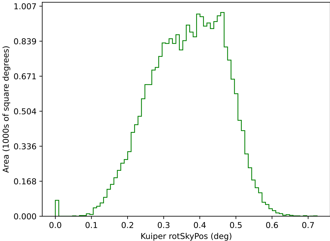
too_combined_s1.0_split_v3.4_10yrs g: Kuiper rotSkyPos
