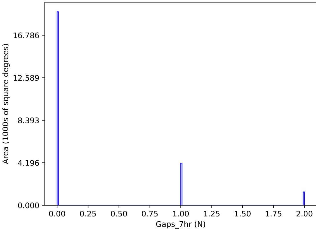
too_combined_s1.0_split_v3.4_10yrs y band: Gaps_7hr
