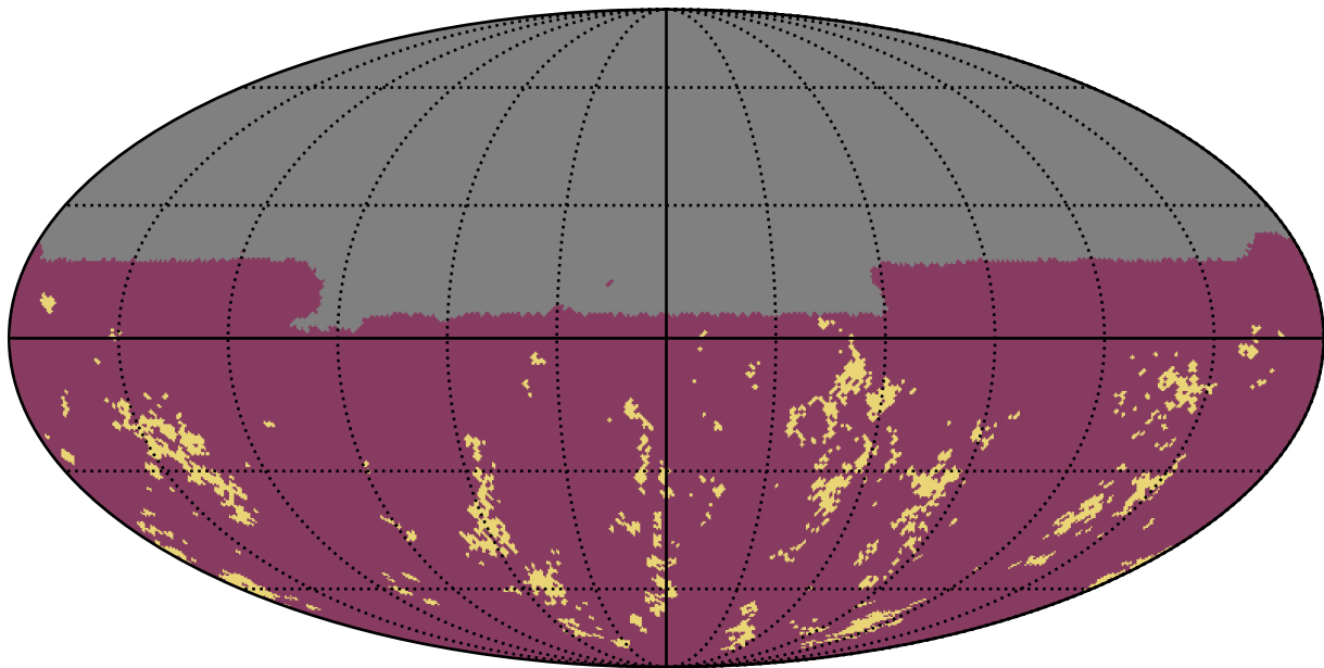
too_combined_s1.0_split_v3.4_10yrs u band: Gaps_7hr
