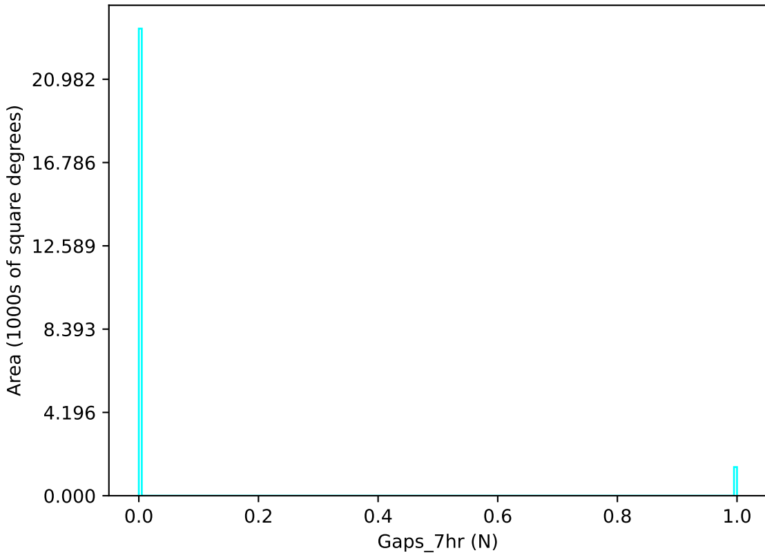
too_combined_s1.0_split_v3.4_10yrs u band: Gaps_7hr
