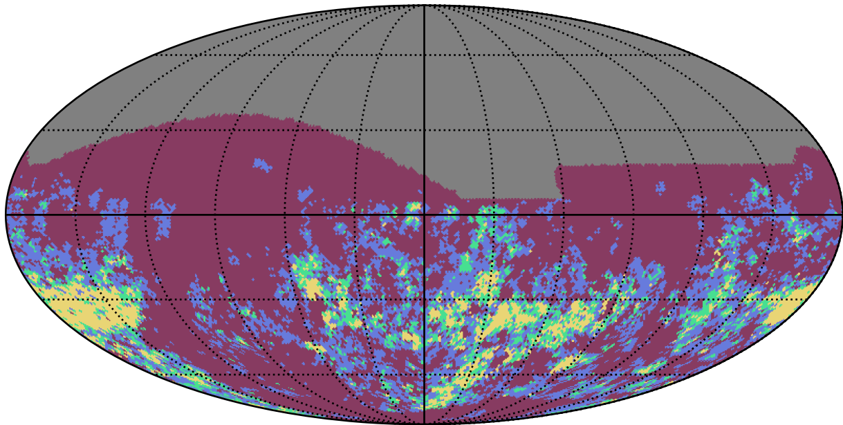
too_combined_s1.0_split_v3.4_10yrs i band: Gaps_7hr
