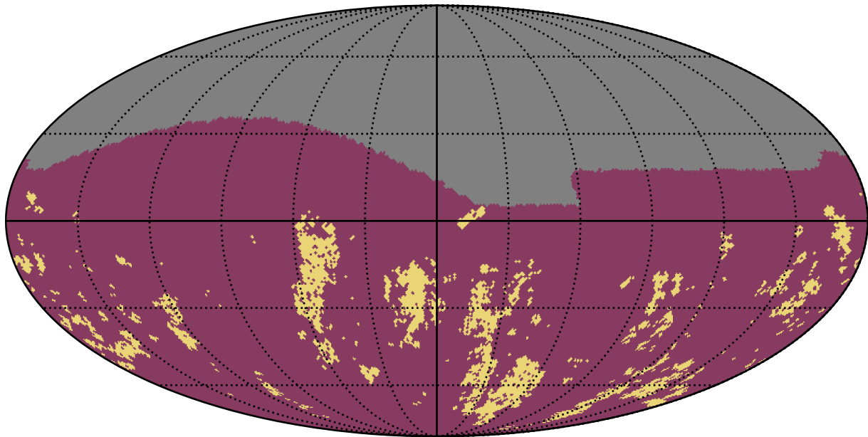
too_combined_s1.0_split_v3.4_10yrs g band: Gaps_7hr
