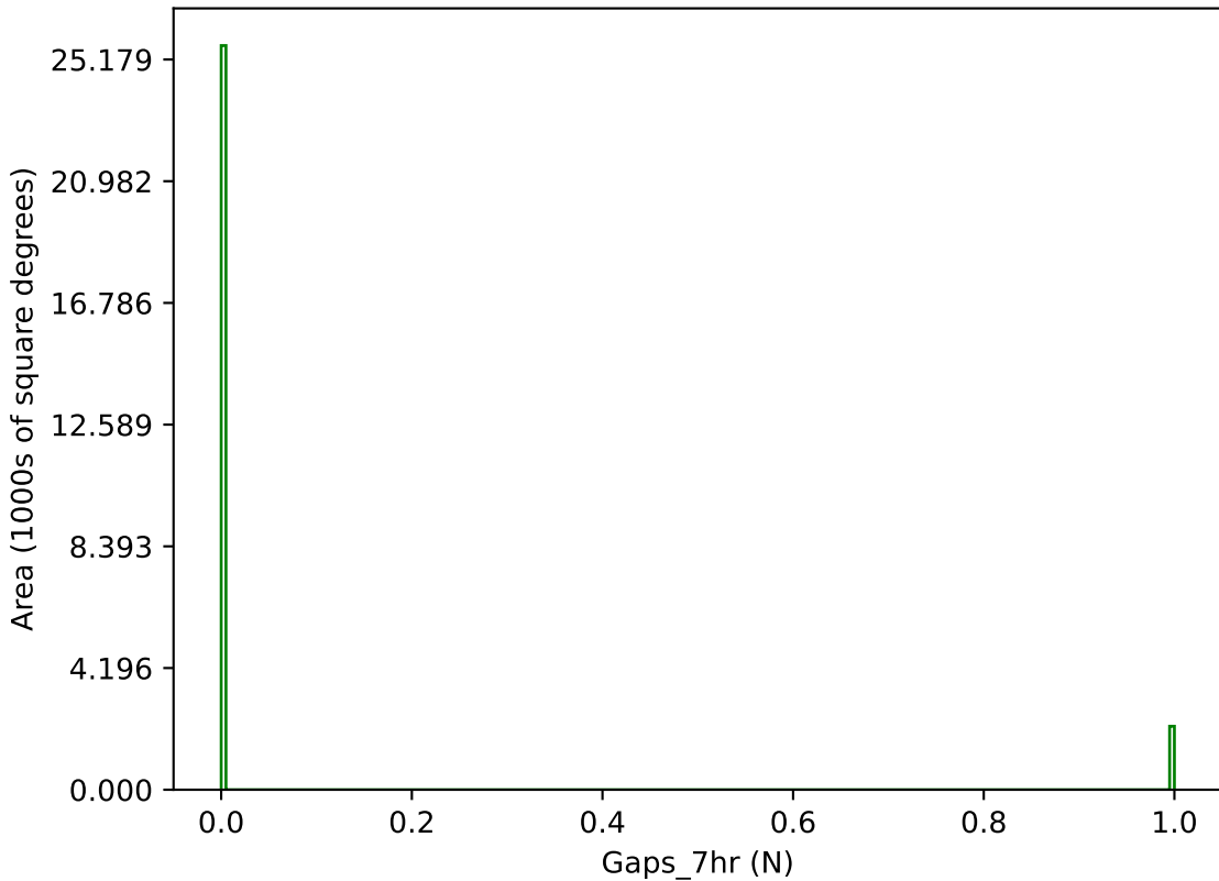
too_combined_s1.0_split_v3.4_10yrs g band: Gaps_7hr
