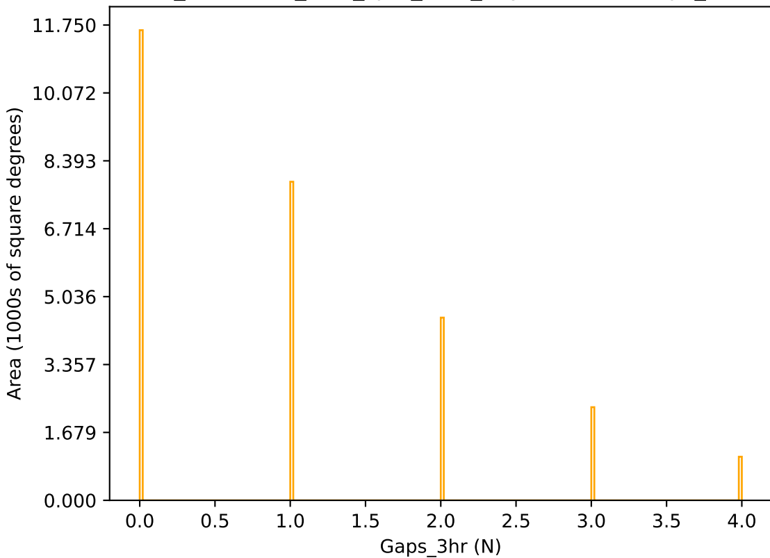
too_combined_s1.0_split_v3.4_10yrs r band: Gaps_3hr
