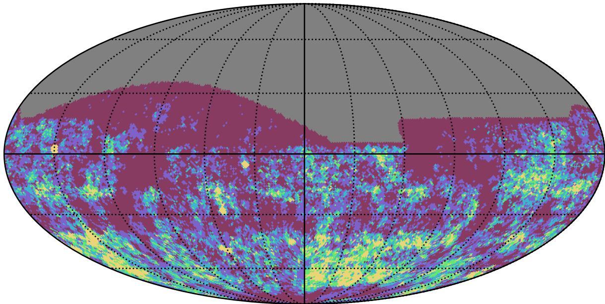
too_combined_s1.0_split_v3.4_10yrs i band: Gaps_3hr
