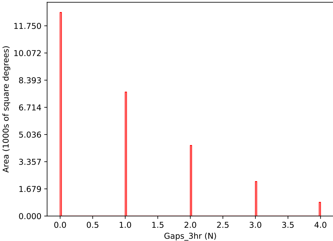
too_combined_s1.0_split_v3.4_10yrs i band: Gaps_3hr
