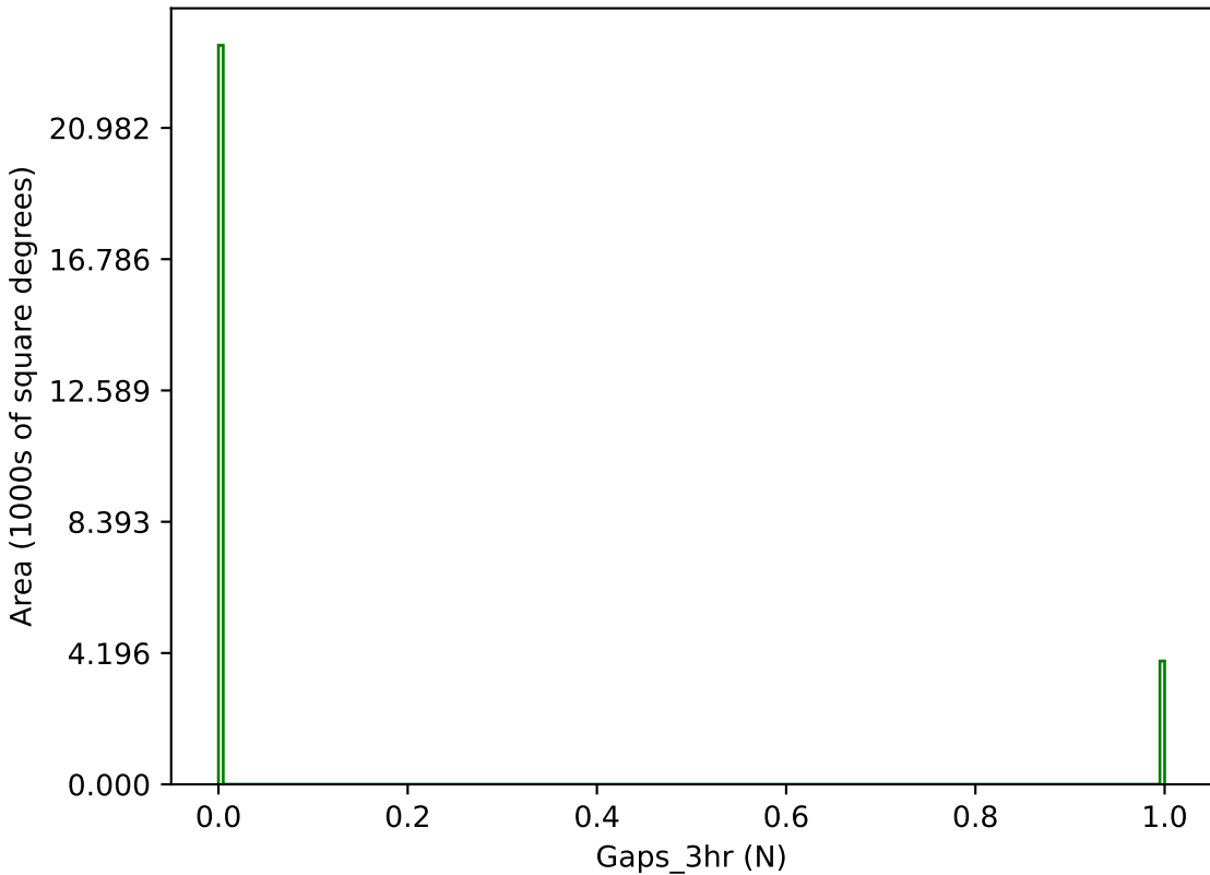
too_combined_s1.0_split_v3.4_10yrs g band: Gaps_3hr
