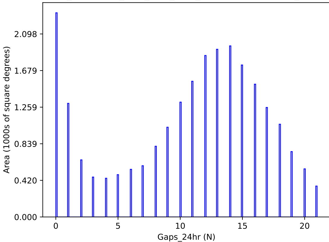
too_combined_s1.0_split_v3.4_10yrs y band: Gaps_24hr
