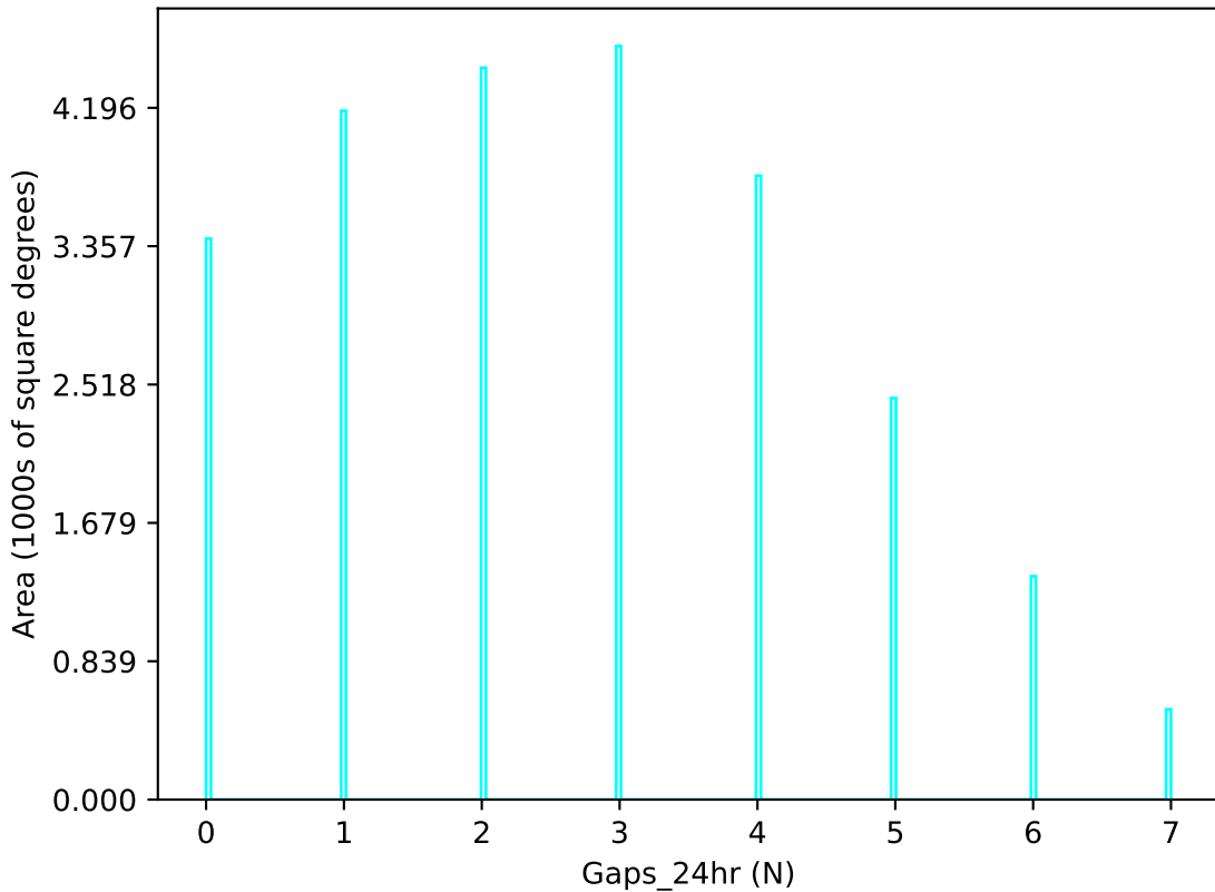
too_combined_s1.0_split_v3.4_10yrs u band: Gaps_24hr
