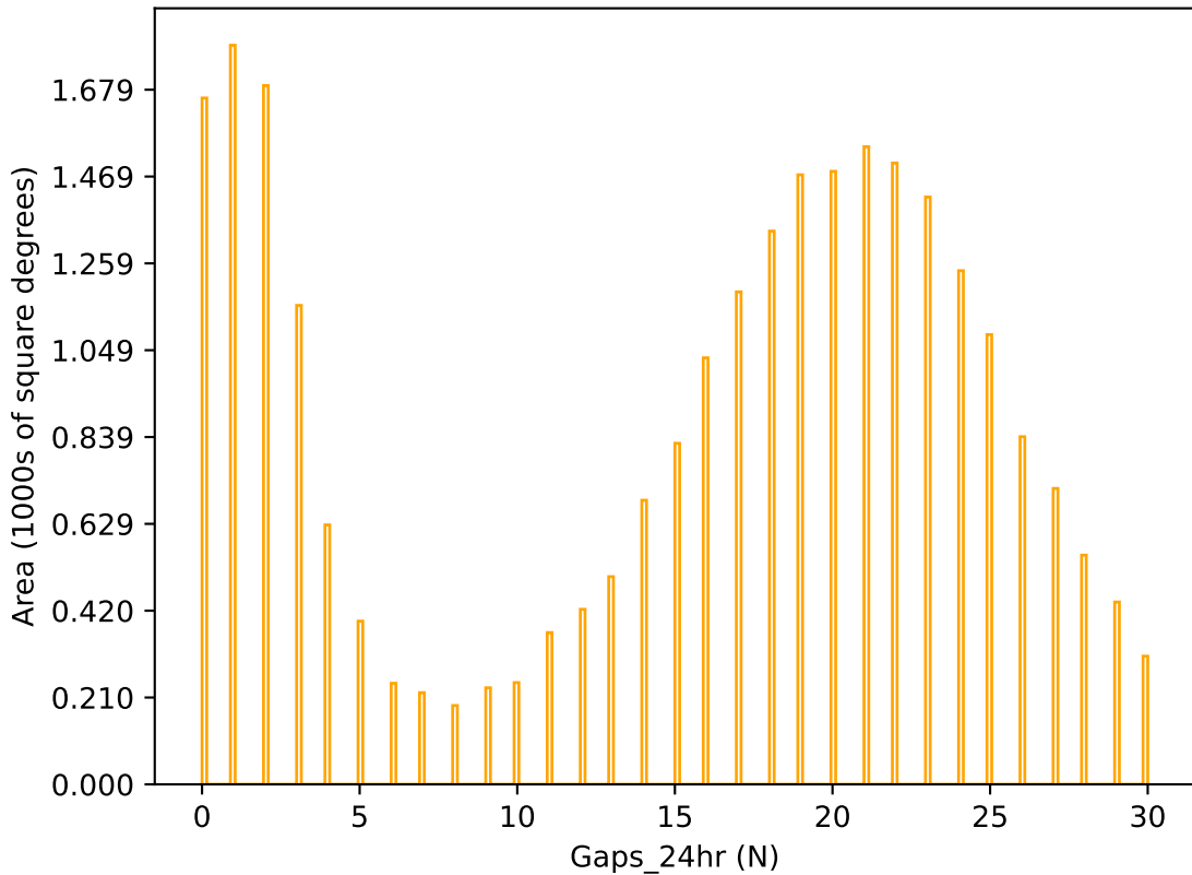
too_combined_s1.0_split_v3.4_10yrs r band: Gaps_24hr
