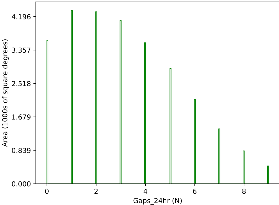
too_combined_s1.0_split_v3.4_10yrs g band: Gaps_24hr
