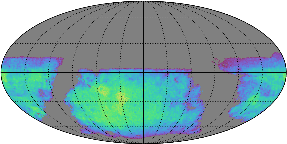
too_combined_s1.0_split_v3.4_10yrs i band non-DD year 8: ExgalM5WithCuts
