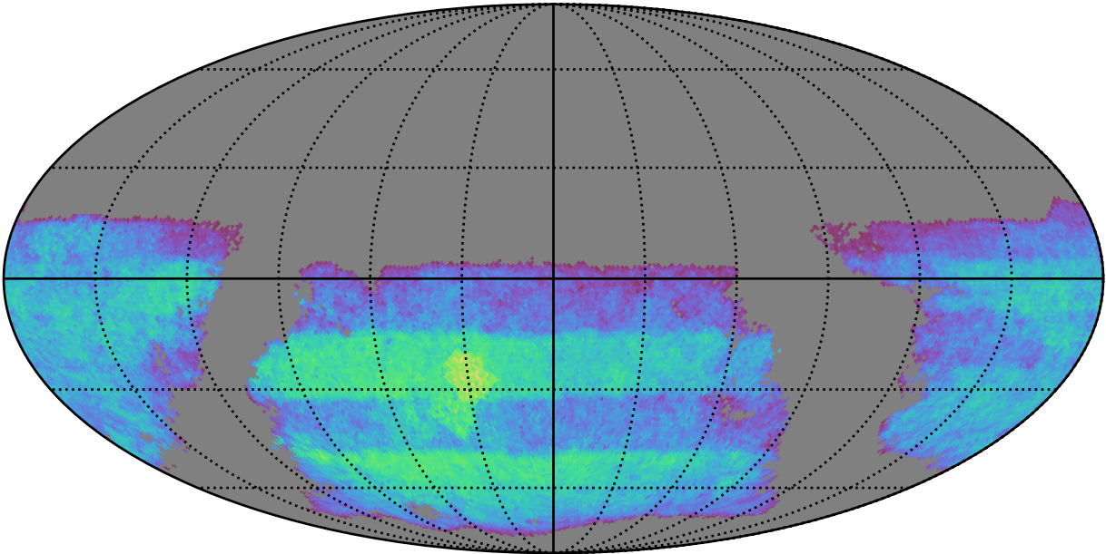
too_combined_s1.0_split_v3.4_10yrs i band non-DD year 3: ExgalM5WithCuts
