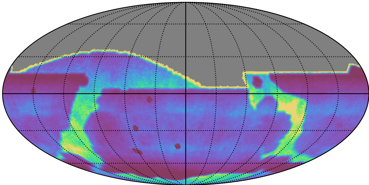
too_combined_s1.0_split_v3.4_10yrs : DCRprecision
