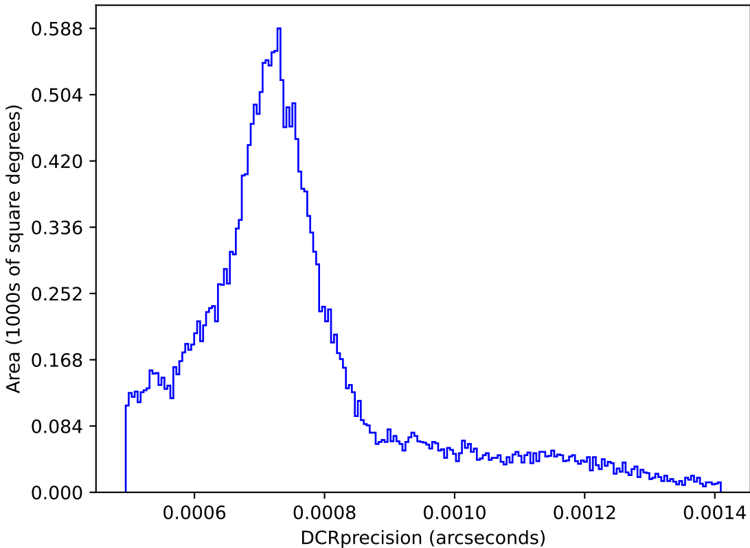
too_combined_s1.0_split_v3.4_10yrs : DCRprecision
