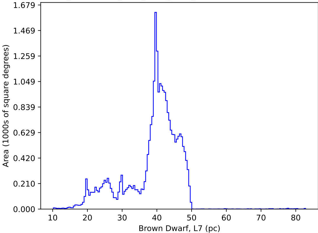
too_combined_s1.0_split_v3.4_10yrs : Brown Dwarf, L7
