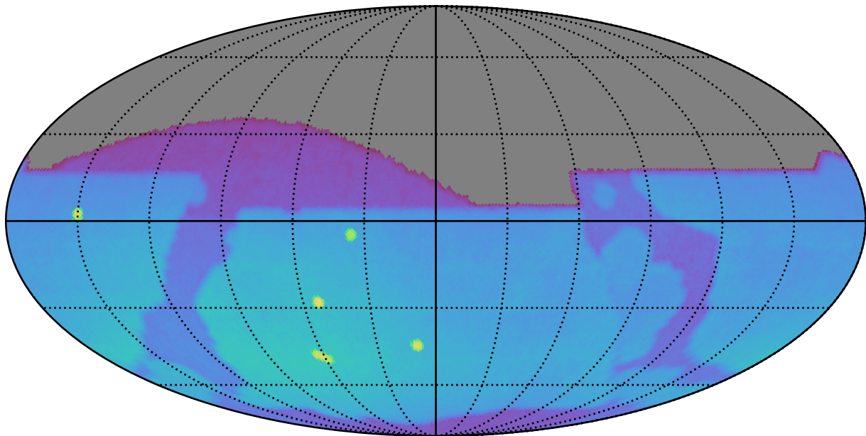
too_combined_s1.0_split_v3.4_10yrs : Brown Dwarf, L4
