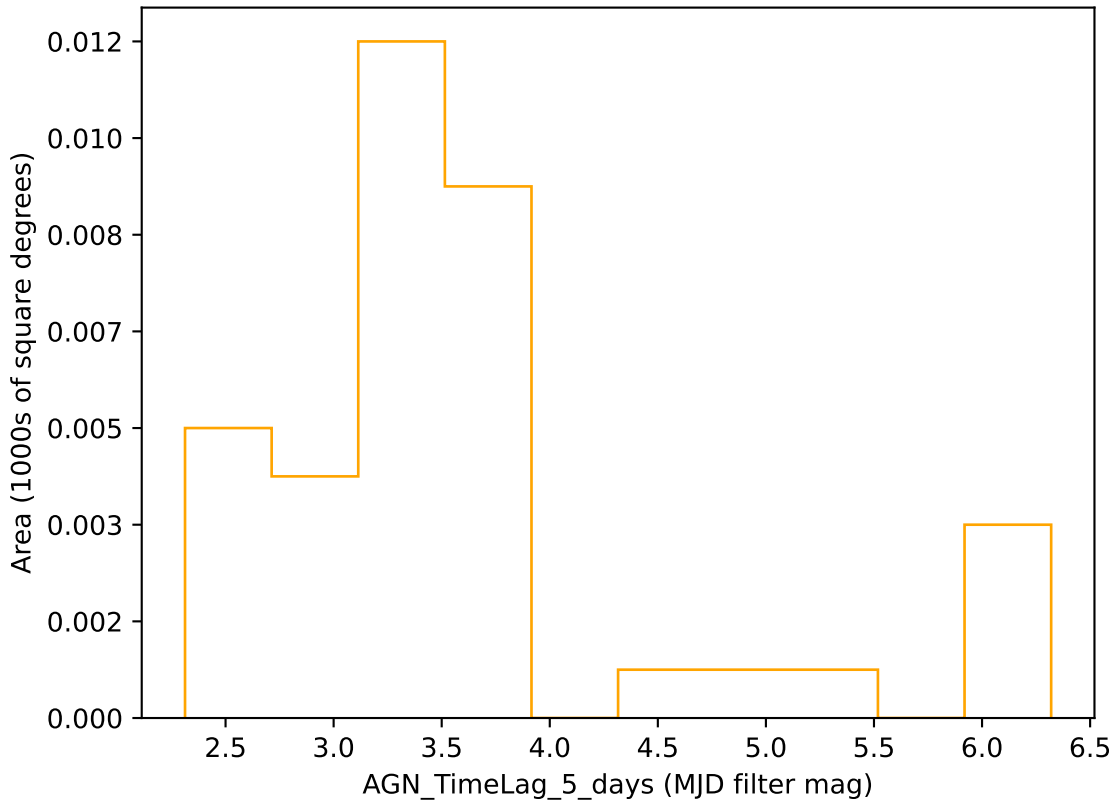
too_combined_s1.0_split_v3.4_10yrs r band: AGN_TimeLag_5_days
